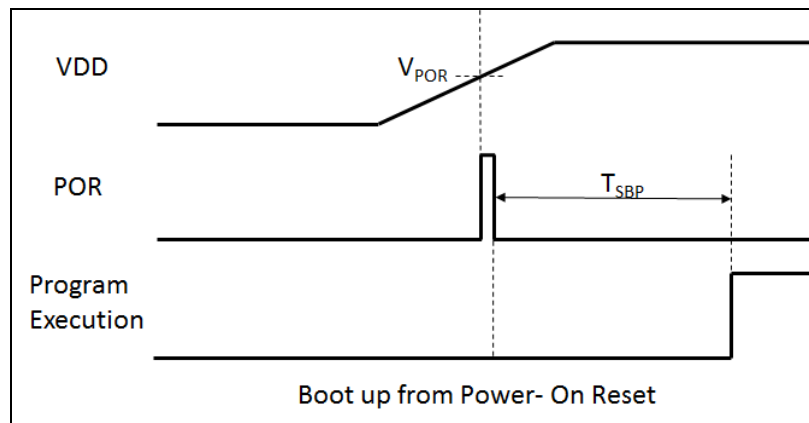
Fig.1: Power-Up Sequence
