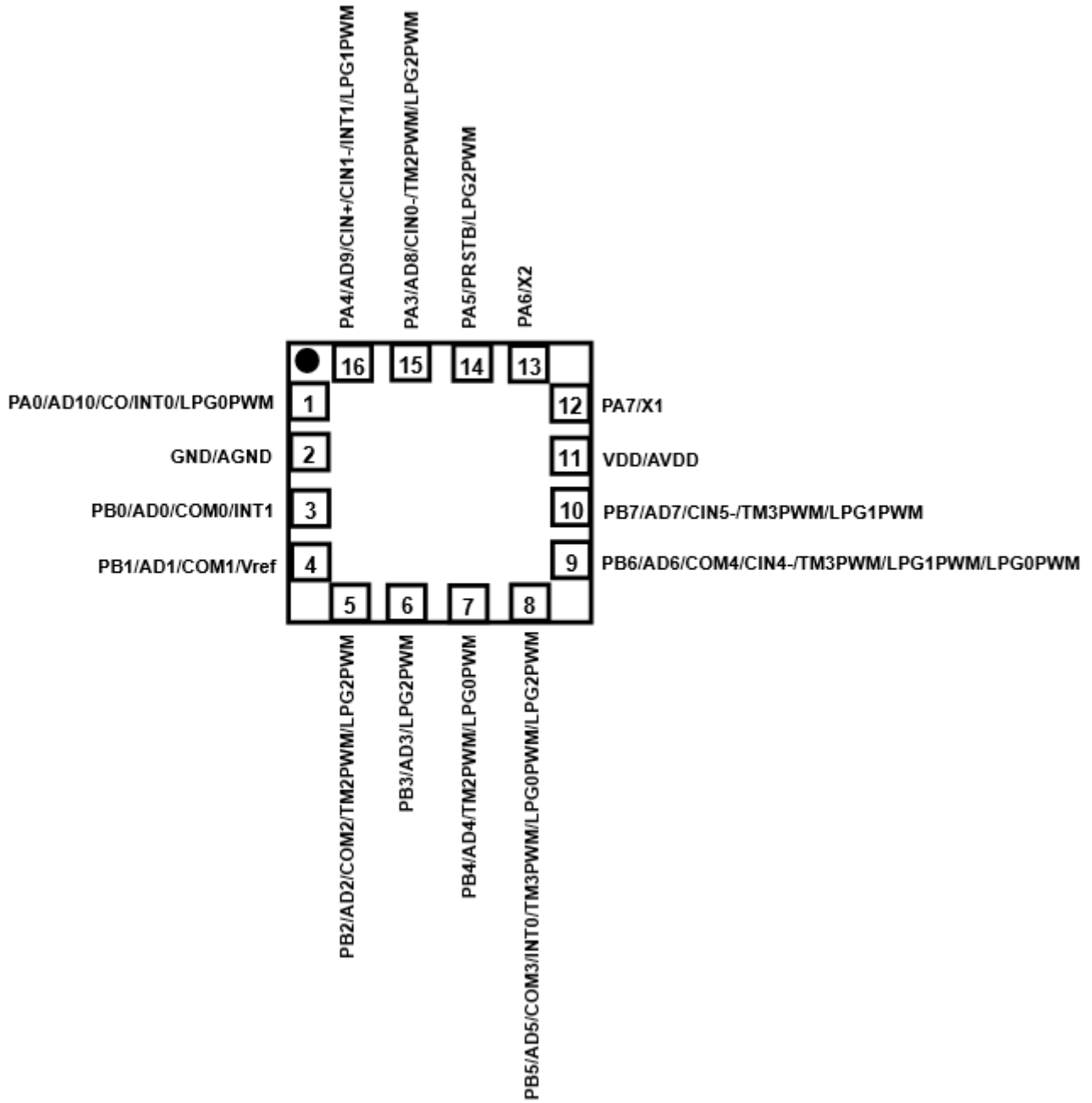
PFS123-1J216A (QFN3*3-16P-0.5pitch)
